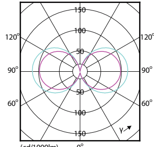
(cd/1000lm) 0° 150° 0-180° 180° 90-270° 150°
