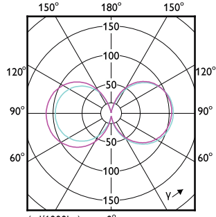
(cd/1000lm) 0° 150° 0-180° 180° 90-270° 150°
