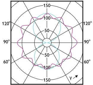
(cd/1000lm) 0° 150° 0-180° 180° 90-270° 150°
